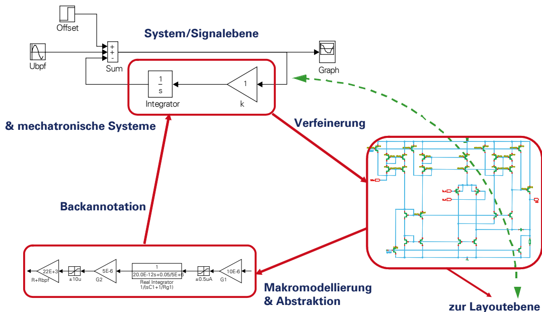
Abbildung 1.5: Mixed-Signal/Mixed-Level Systembeschreibung
